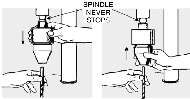
1. Grip Sleeve. Pull down. Jaws open automatically; drill is released.
